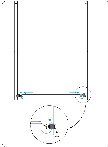
Step 2: Fasten the bottom crossbar with the help of large plastic screws.
