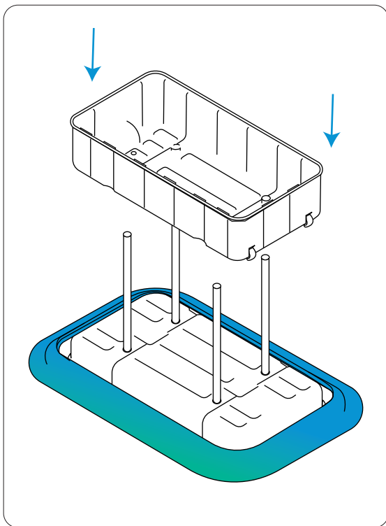
Step 3: Place the bottom piece of the case on top.
